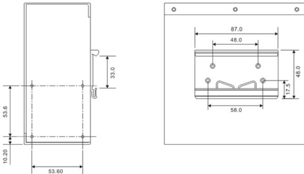
DIN-rail Kit Measurement
