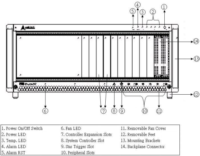
Figure 1-1 Front View of the PXIS-2630 Chassis
