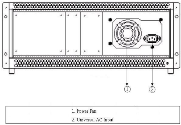
Figure 1-2 Rear View of the PXIS-2630 Chassis
