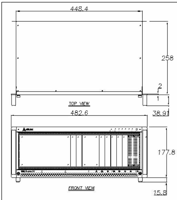
Figure A-1 PXIS-2630 Dimensions
