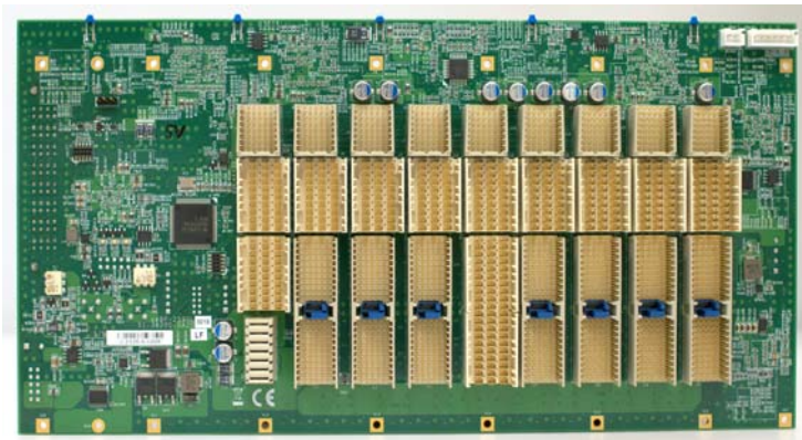
Figure 1-9: PXES-2590 Backplane
