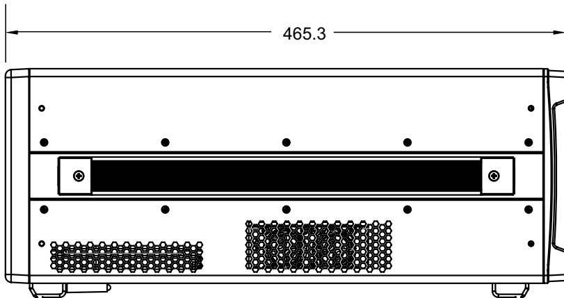
Figure 1-1: Front View
