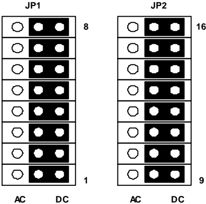
Figure 2.2 Default Input Signal Jumper Setting
