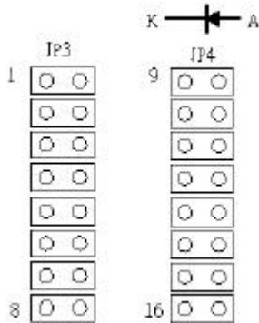
Figure 2.3 External LED connectors for relay status indication
