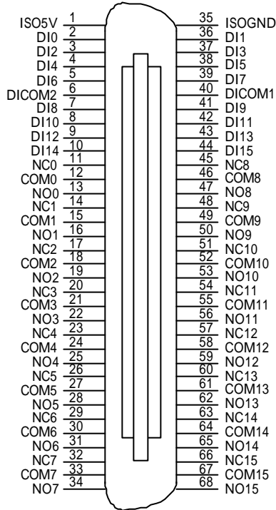
Figure 2.5 Pin Assignment of PCI-7256 CN1
