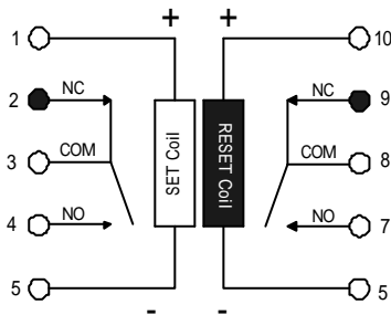
Figure 4.1 2 coil latching relay(RESET condition)
