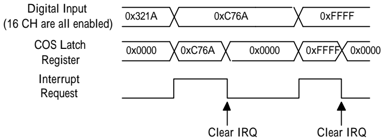
Figure4.4 Timing of COS
