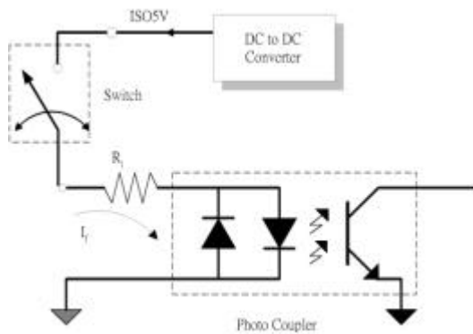
Figure 4.3 Dry contact
