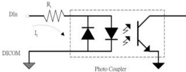
Figure 4.2 Photo Coupler
