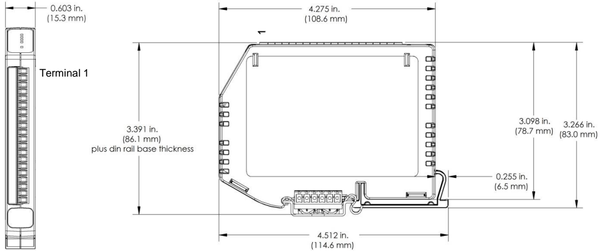
Figure 1: Module Dimensions
