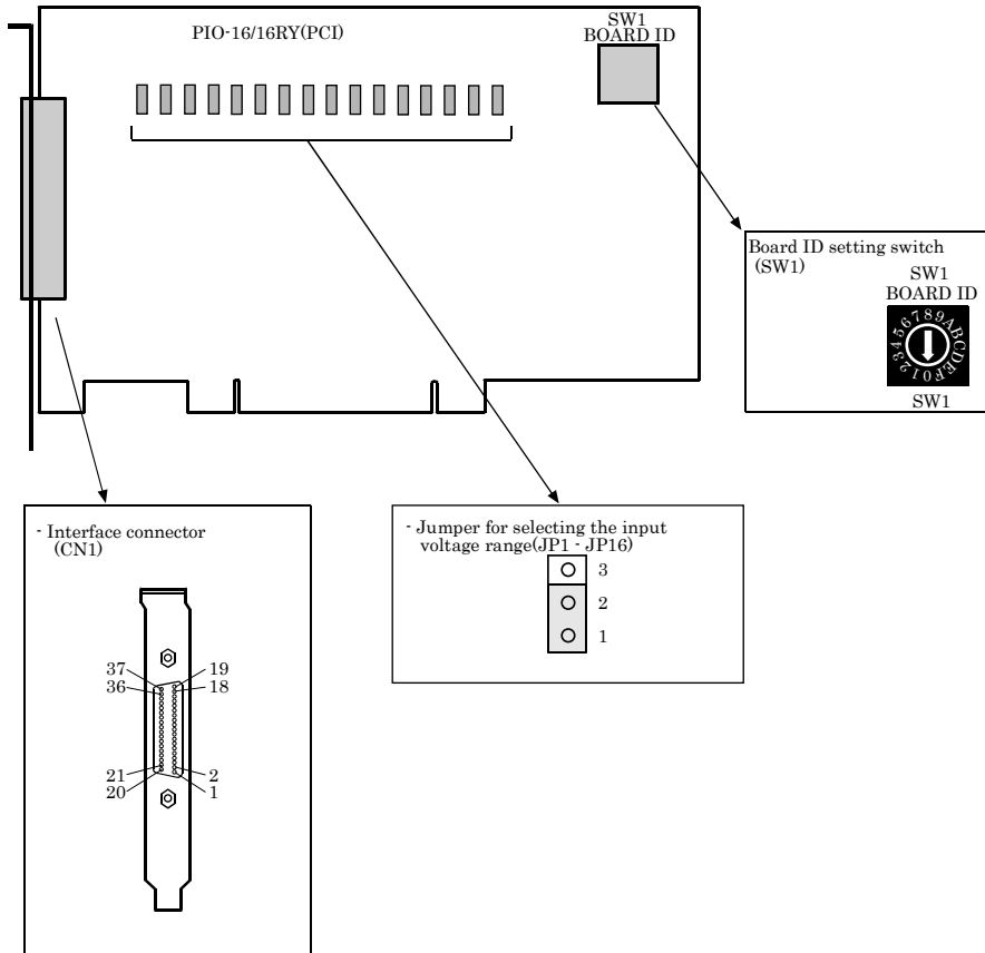
Figure 2.1. Component Locations
