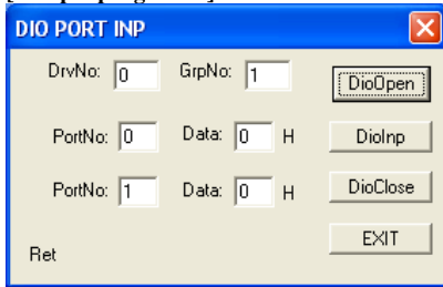
[Sample program 1]
