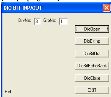
[Sample program 5]
