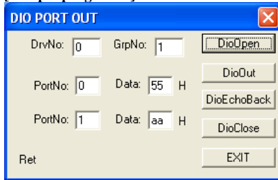
[Sample program 2]
