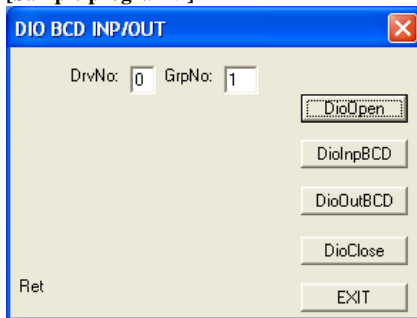
[Sample program 9]
