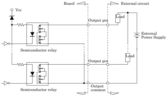
Figure 3.7. Output Circuit
