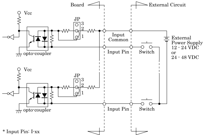
Figure 3.3. Input Circuit
