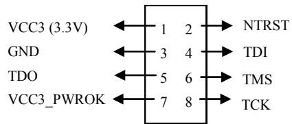
CON1 JTAG Connector
