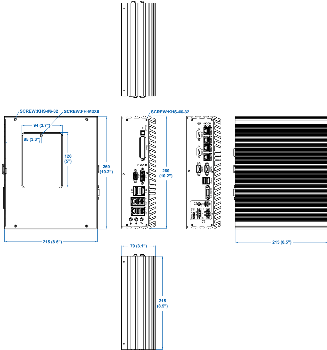
Figure 1.1 ECS-7800-PoE
