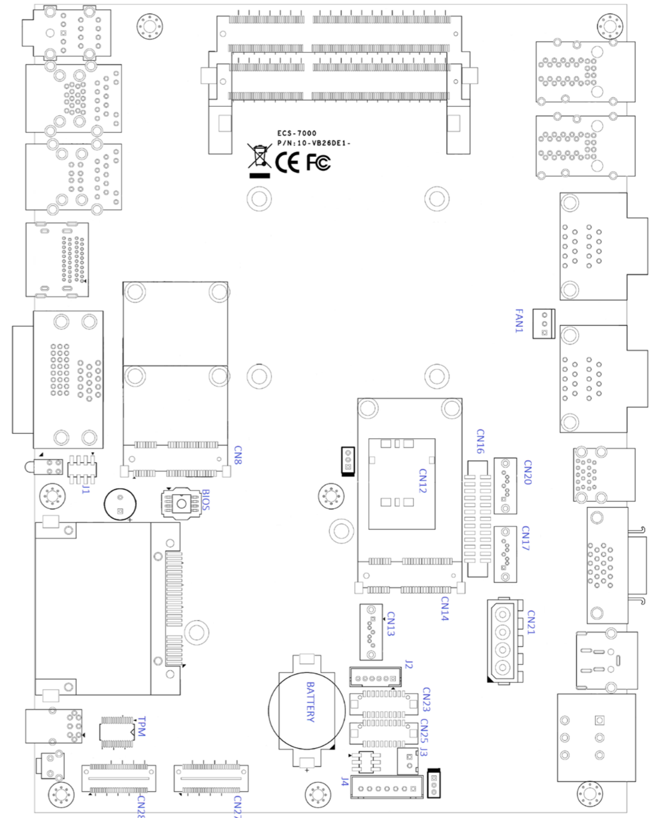
Figure 2.3.1 Internal Connectors and Jumpers
