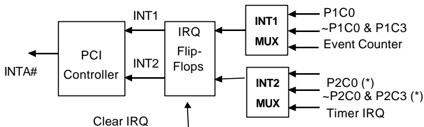
Fig 4.3 Dual Interrupt System of PCI-7224/7248/96
