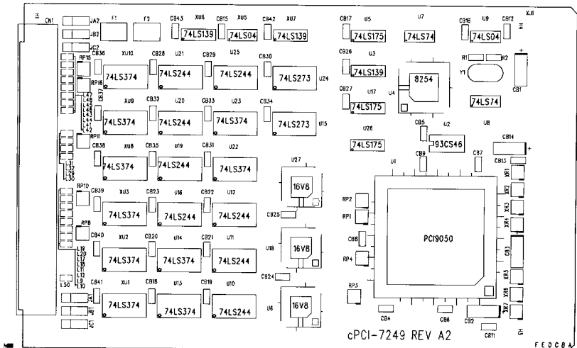
Figure 2.3.4 cPCI-7249R Layout
