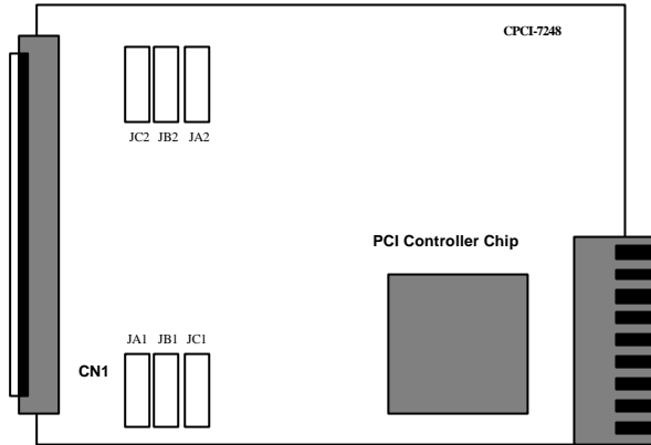
Figure 2.3.3 cPCI-7248 PCB Layout
