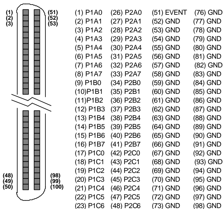
Figure 2.6.2 pinout and power signals of cPCI-7248
