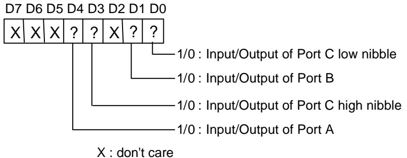
Figure 4.1 Control Word Format
