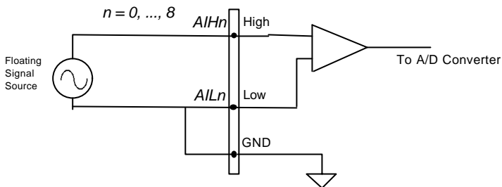
Figure 4.1.4 Floating source and differential input
