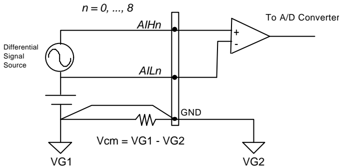
Figure 4.1.3 Differential source and differential input
