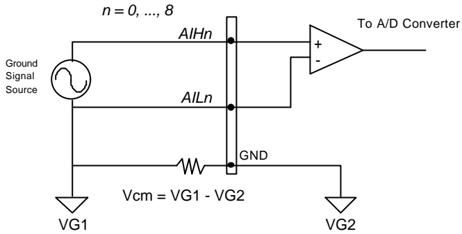
Figure 4.1.2 Ground source and differential input
