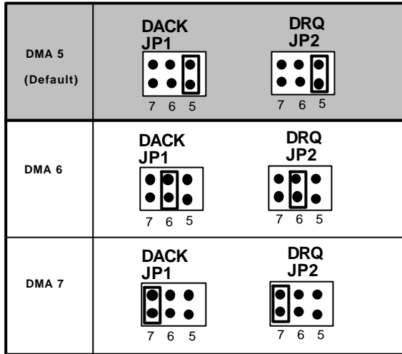
Figure 2.7 DMA Channel Setting
