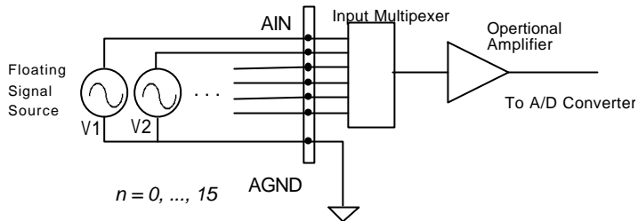
Figure 4.1.1 Floating source and single-ended
