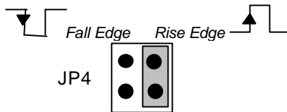
Figure 2.6 Jumper JP4 setting
