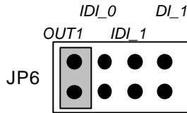
Figure 2.5-2 Jumper JP6 setting
