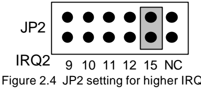
Figure 2.4 JP2 setting for higher IRQ
