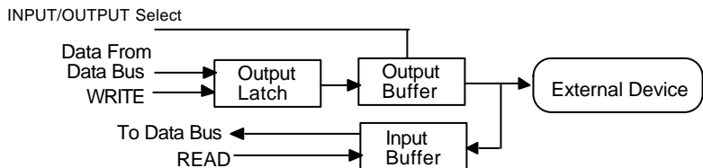
Figure 3.1 ACL-7122's Signal Direction
