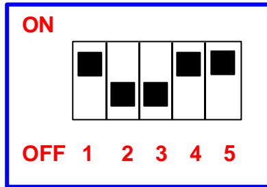
Figure 2.3 Default Switch Setting
