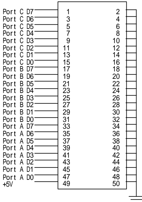
Figure 2.5 Connector Pin Assignment
